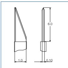
H-1393/3 Arcurate (Thornton)
